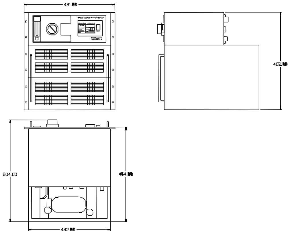
(c) S4000 RS Enclosure Outline Drawing
