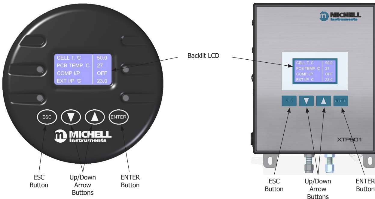
Figure 4 User Interface
