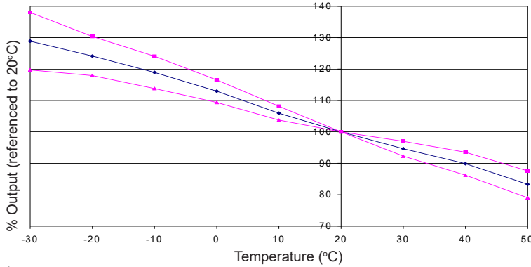
Figure 1 Sensitivity Temperature Dependence
