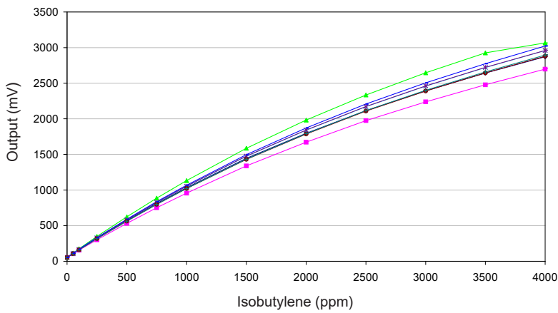
Figure 2 Linearity to Isobutylene
