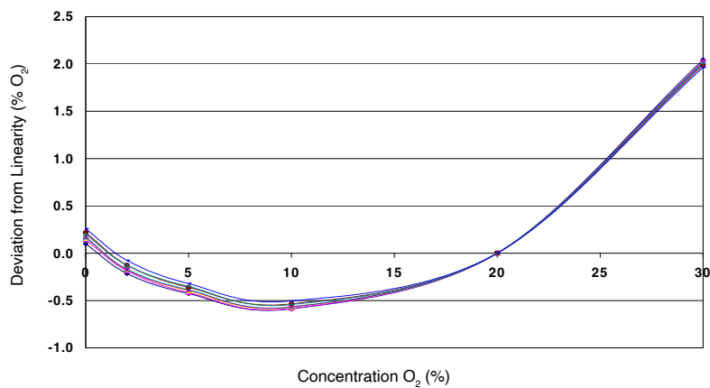
Figure 3 Linearity
