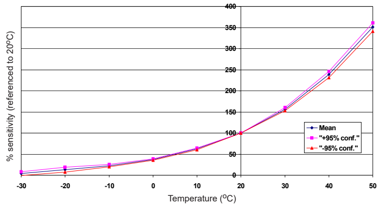
Figure 2 Hydrogen Sensitivity Temperature Dependence
